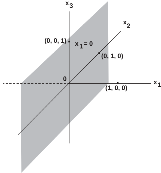
Figure 3.22: The x_2, x_3 -coordinate hyperplane represented by the equation x_1 = 0 in R^3 .
