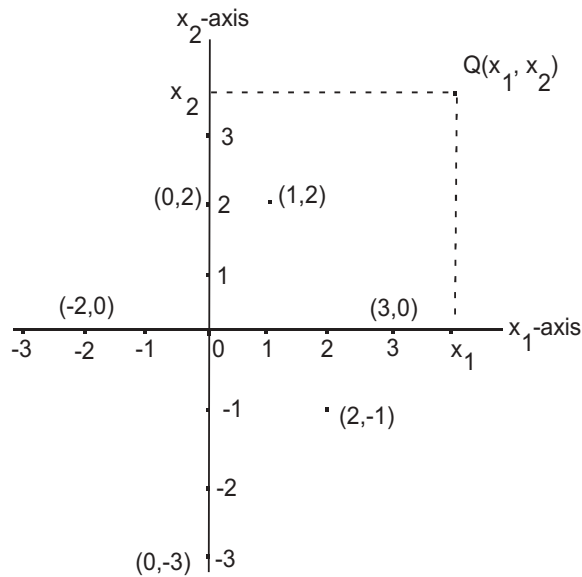
Figure 3.2: The Cartesian (rectangular) coordinate system for the 2-dimensional plane. The angles are all 90^\circ ( \pi/2 in radians). 2-dimensional vectors x = (x_1, x_2) are represented as points in the 2-dimensional plane.
