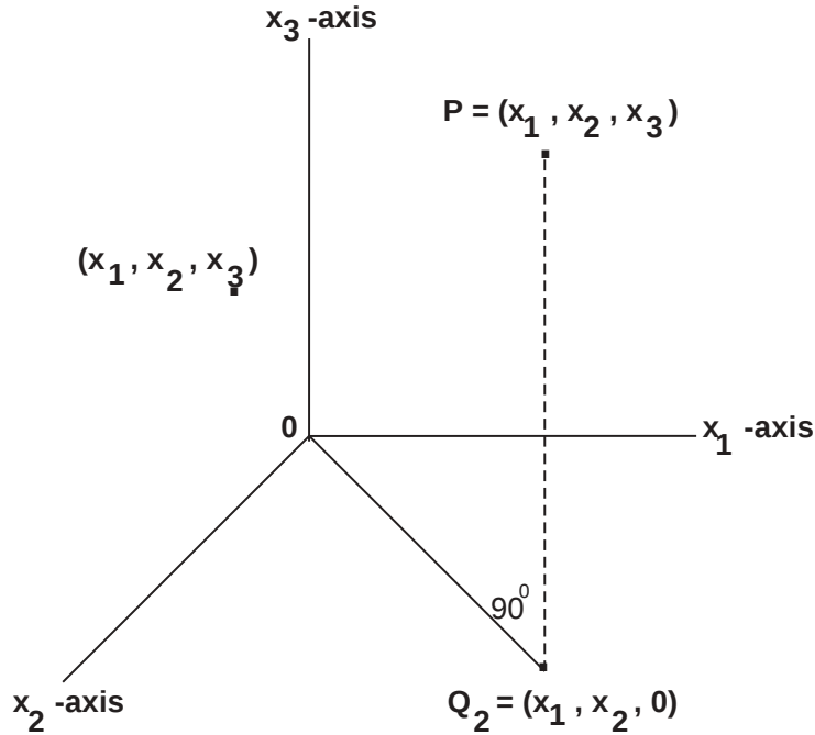
Figure 3.32: Euclidean distance function in R^3 explained.
