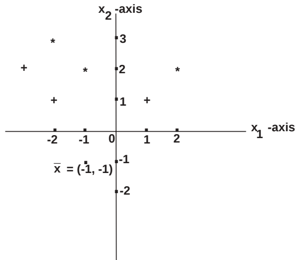
Figure 3.6: The set S consists of all the points marked with “*”. \bar{x} is the point marked with “.”. \bar{x} + S is the set of all points marked with “+”.
